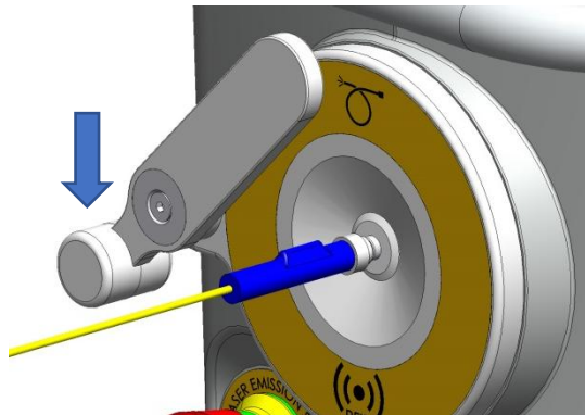
Fig. 4-5: Connection of the fiber (ELIOS probe)
